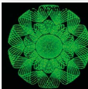
Anti-stokes
