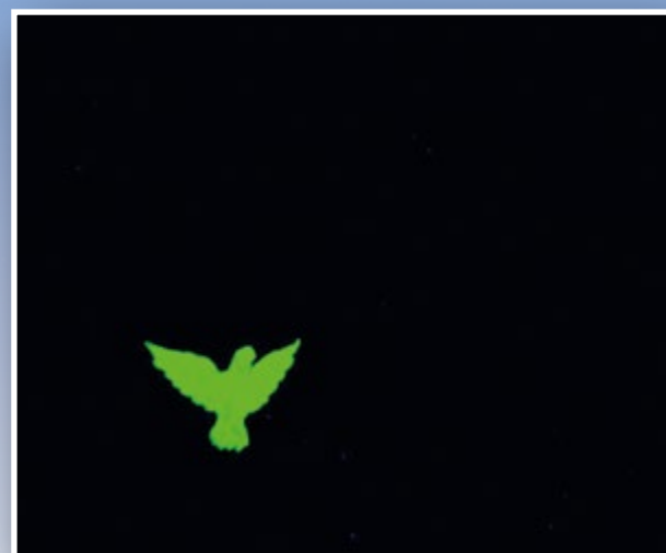
anti-Stokes
