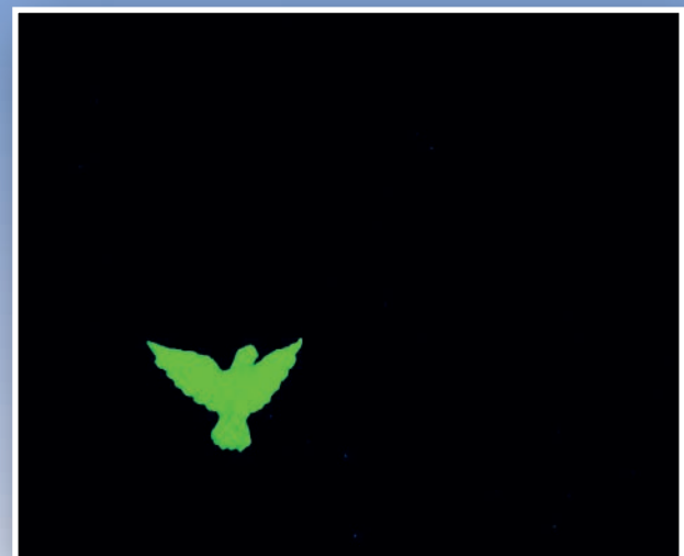
anti-Stokes
