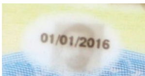
CLI feature
